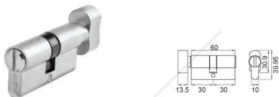
CYL BK DL60MM SN
