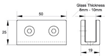
GLASS CLIP U820 PSS Glass to wall applications
