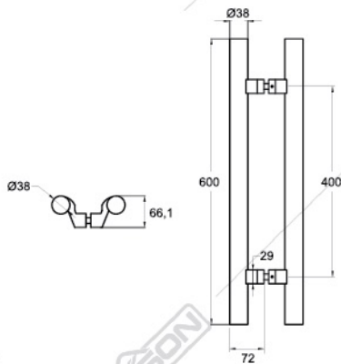
PH DL810 38x600x400 PSS+SSS Available in : 38x800x600 PSS+SSS 38x1000x800 PSS+SSS
