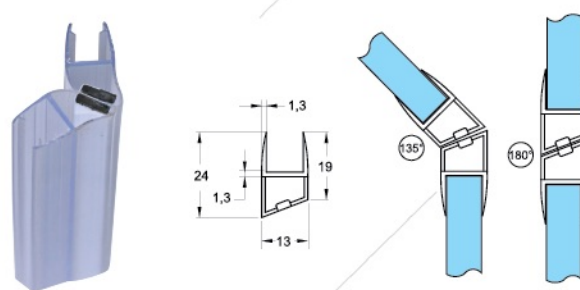
CLIP SEAL MAGNETIC CS 110 10x2.2M (135/180) WH
