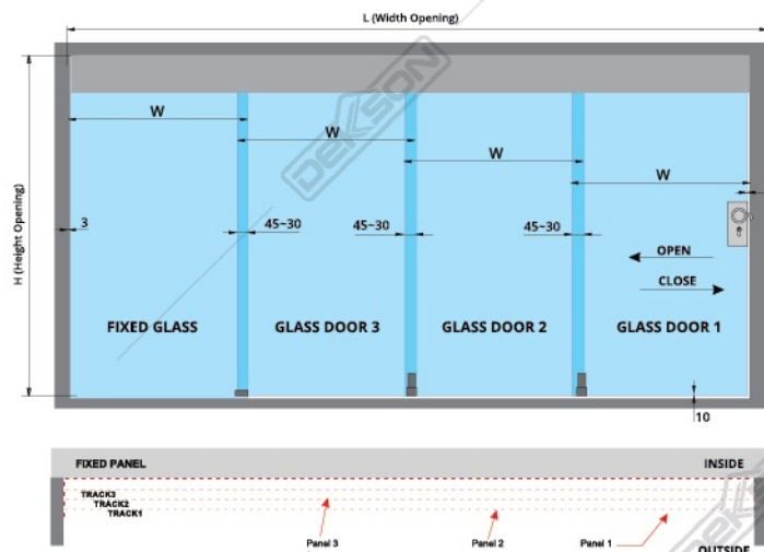
DOOR PANEL TRACK SGT 4100 (3+1) NA (2 pc)
