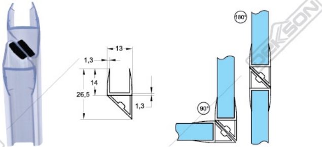
CLIP SEAL MAGNETIC CS 100 10x2.2M (90/180) WH
