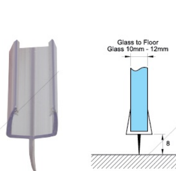
CLIP SEAL BS (10/12MM) 2.5M*
