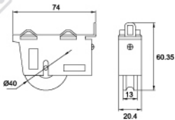
RSD 001 HD Capacity (Max.) : 75 Kg / pair
