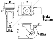
RC 250 50MM BRAKE Capacity (Max.) : 50 Kg / pair
