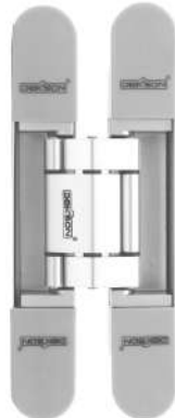
CONCEALED HINGE ES CONC D80 NA Available : Matt Black Capacity (max) : 80 KG / pair Max. Door Width: 90 cm Opening Angle : ≤ 150°
