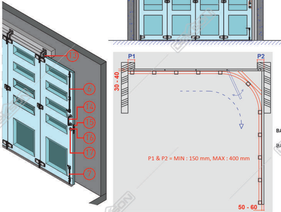
13 MORTISE SLIDING
