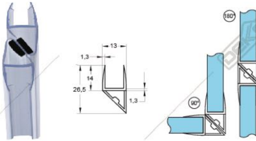
CLIP SEAL MAGNETIC CS 100 10x2.2M (90/180) WH
