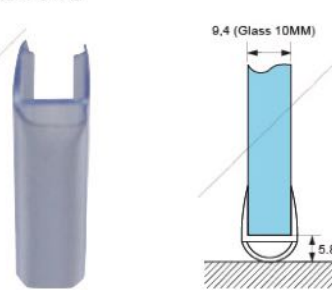
CLIP SEAL CS 8920 10x2.2M OVAL
