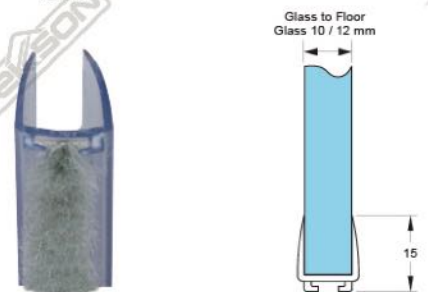
CLIP SEAL WITH BRUSH CSB 002 10x2.2M OVAL* Available : 12x2.2M* 12x3M*
