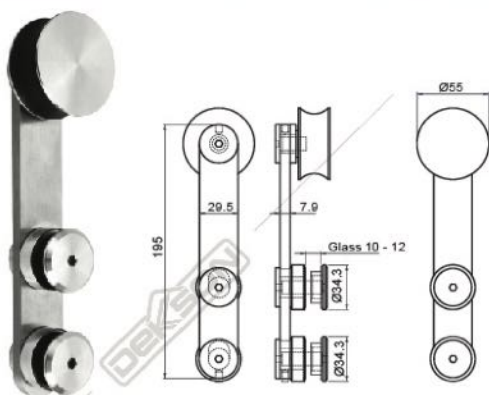
ROLLER FOR TUBE (2 pcs)
