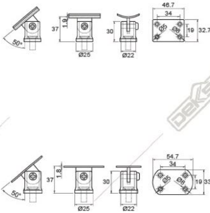
SCH 01 OVAL SSS
