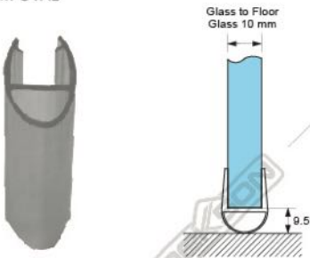
CLIP SEAL CS 8910 10x2.2M OVAL
