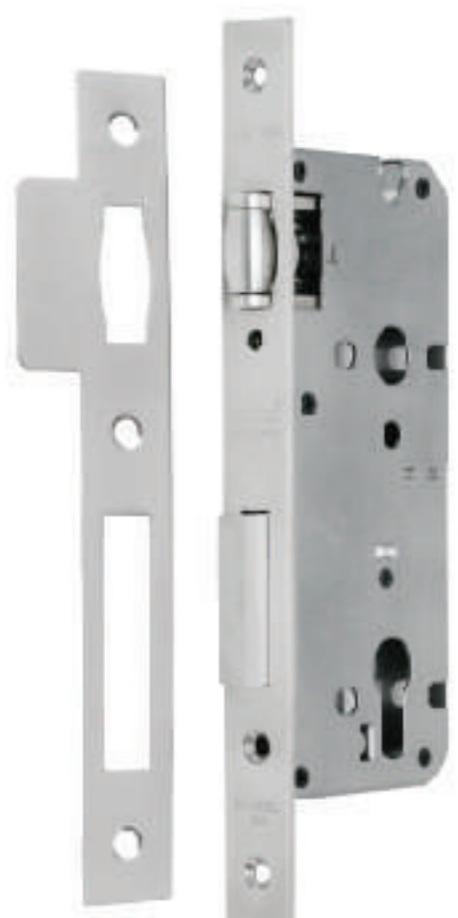
9 MORTISE ROLLER
