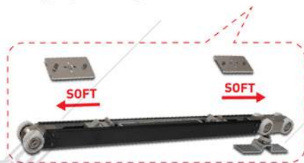
DBL ACT SOFT (Close + Open) SCO 8020 2M Capacity Max. : 80 kg
