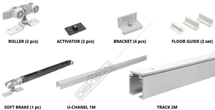
SOFT BRAKE (1 pc) U-CHANNEL 1M TRACK 2M
