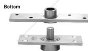
ESS PV 002 SSS Capacity (max) : 250 kg / set
