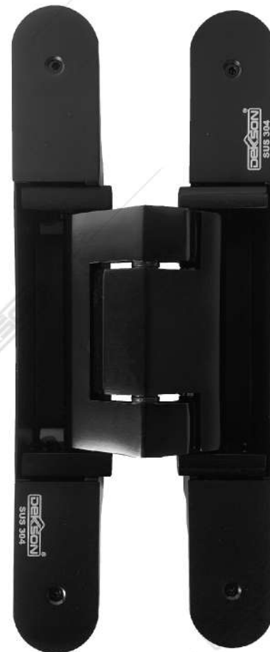
ESS CONC GD200N MATT BLACK Available : SSS Capacity (max) : 200 kg / pair Max. Door Width : 95 cm Opening Angle : \leq 180^\circ
