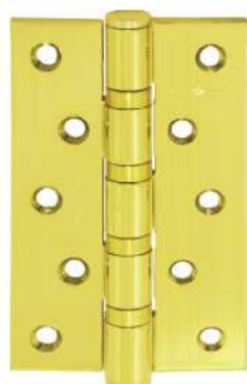
ESS EL 5x3X3MM 4BB TP Capacity (max) : 80 kg / pair
