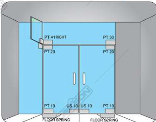
PT 41 PSS RIGHT Available : Left PT 41 MATT BLACK Available : Left or Right
